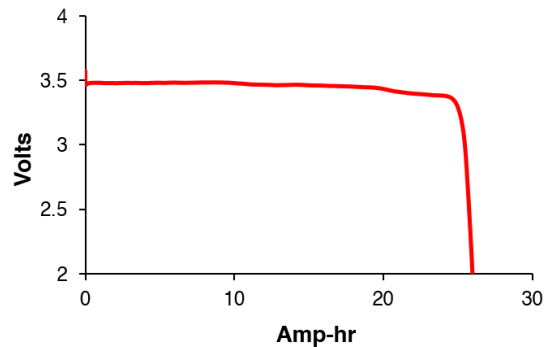
Discharge Curve 200 mA, 23°C
