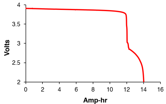
Discharge Curve 50 mA, 120°C
