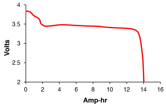
Discharge Curve 175 mA, 23°C
