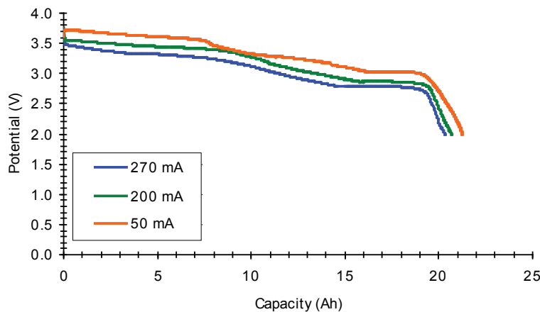
Discharge at 200°C
